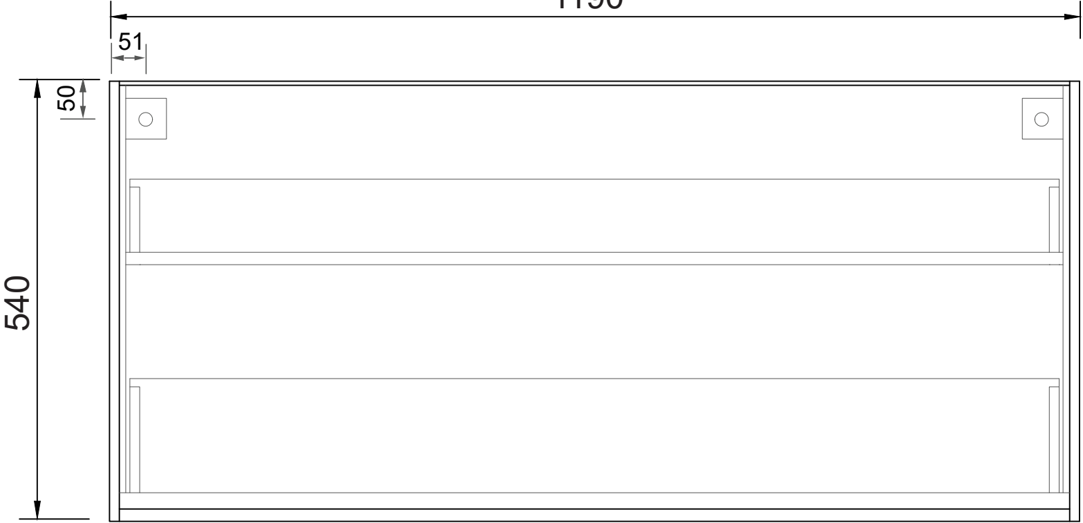
FRONT ELEVATION
