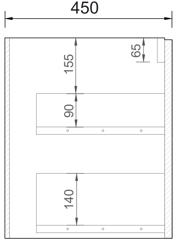
SIDE CROSS-SECTION
