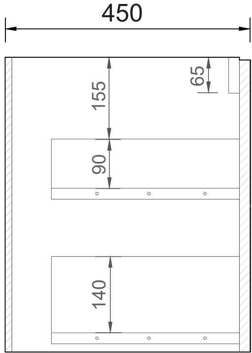
SIDE CROSS-SECTION
