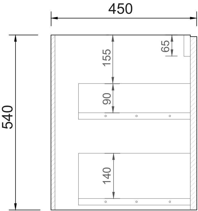
SIDE CROSS-SECTION
