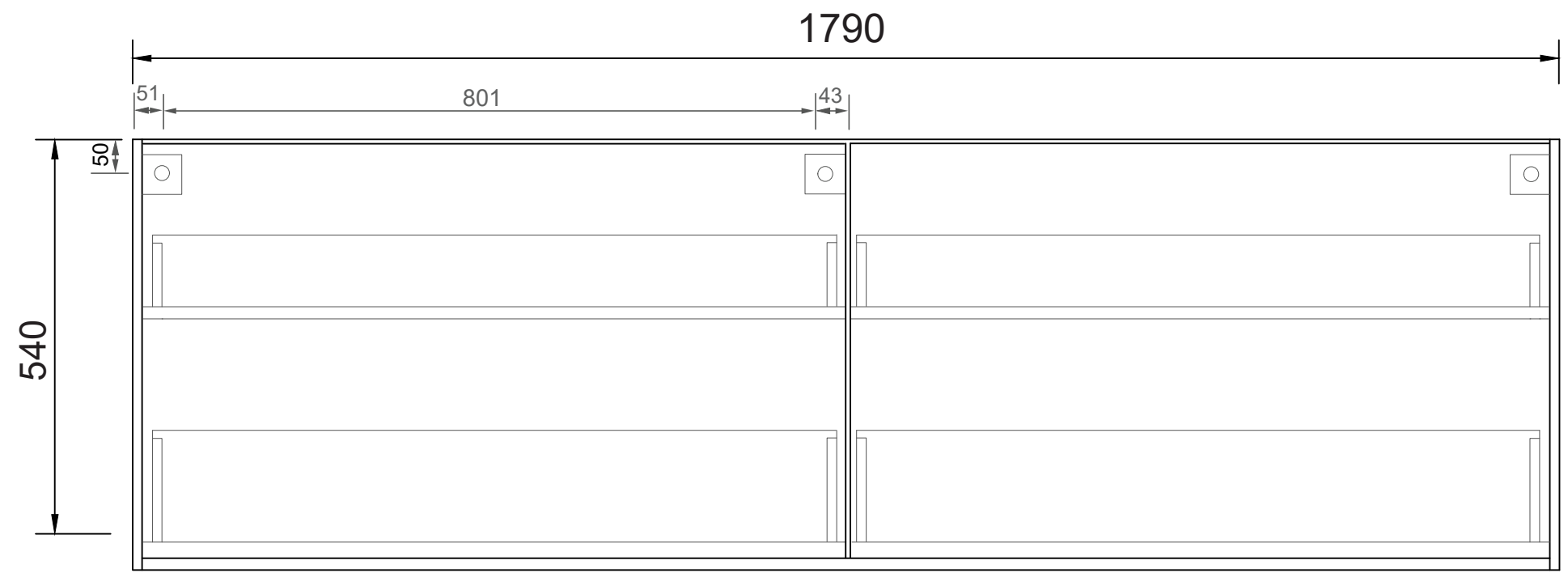
FRONT ELEVATION
