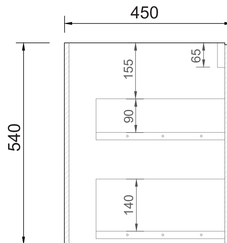
SIDE CROSS-SECTION
