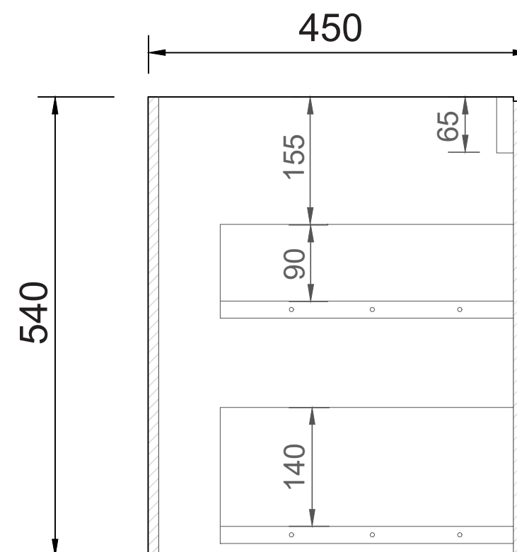
SIDE CROSS-SECTION
