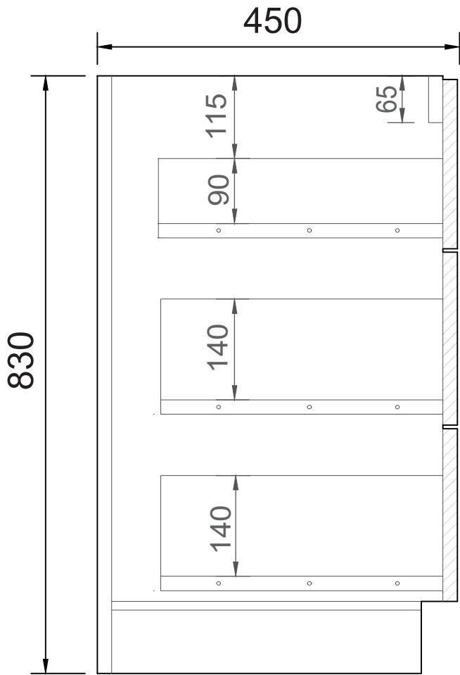
SIDE CROSS-SECTION
