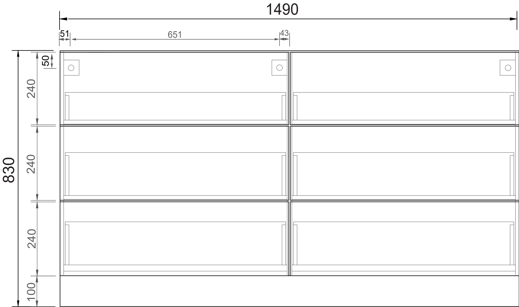
FRONT ELEVATION
