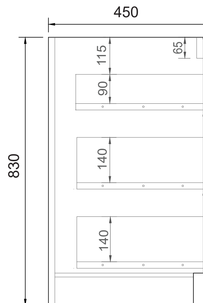
SIDE CROSS-SECTION
