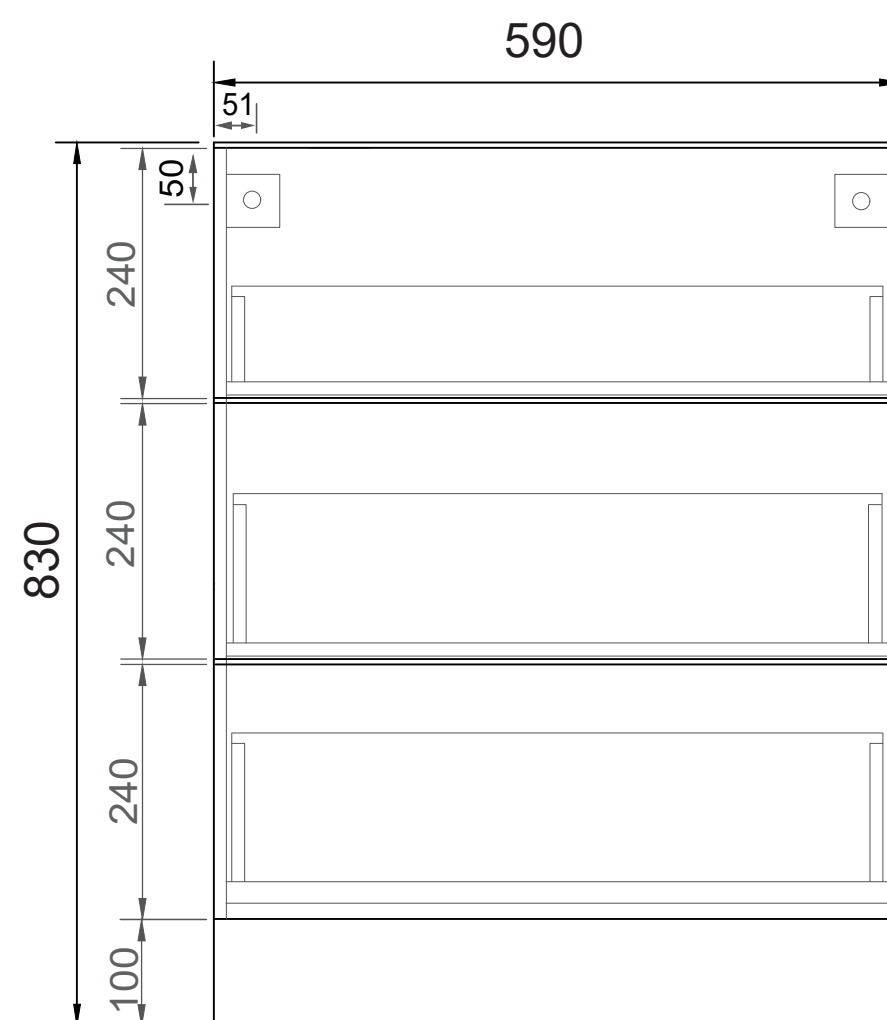
FRONT ELEVATION
