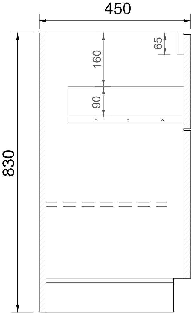
SIDE CROSS-SECTION
