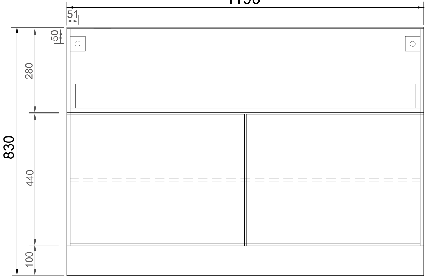
FRONT ELEVATION
