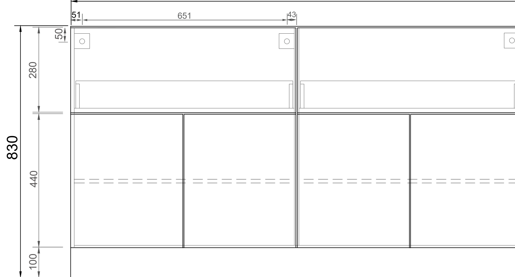
FRONT ELEVATION
