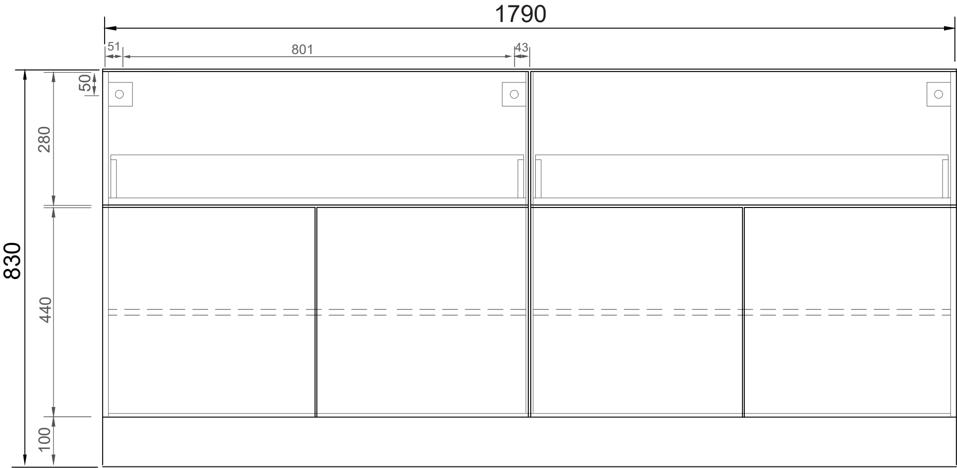
FRONT ELEVATION
