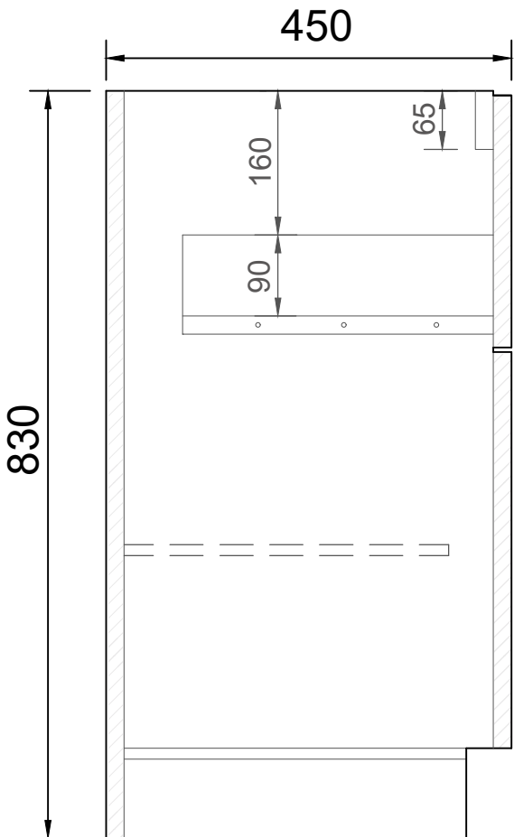
SIDE CROSS-SECTION
