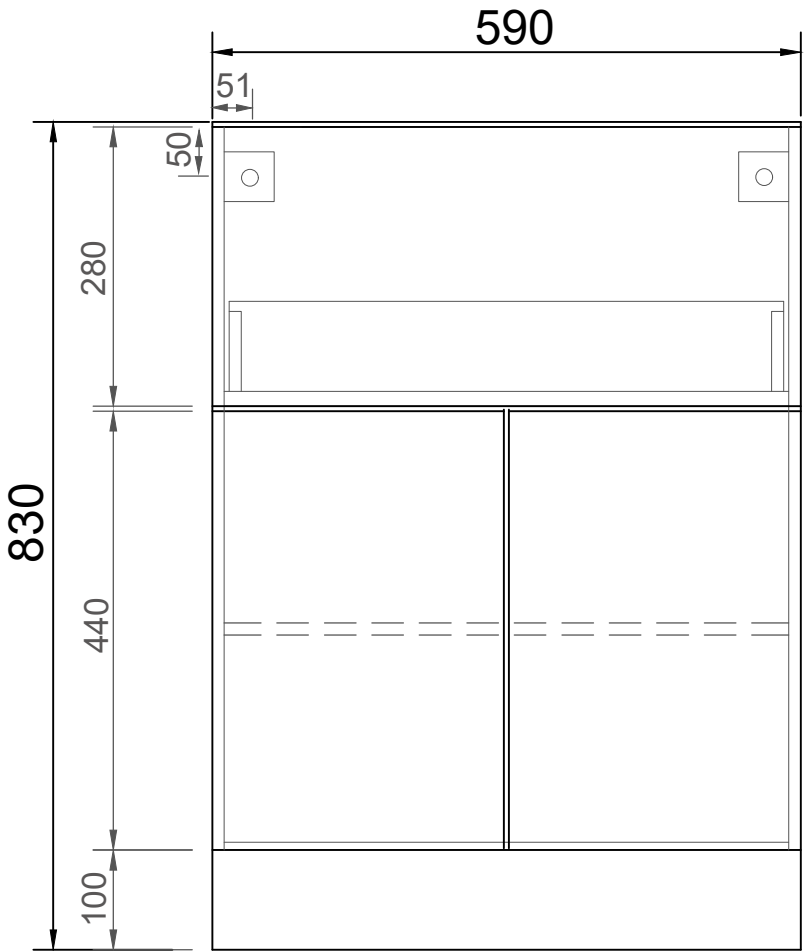
FRONT ELEVATION
