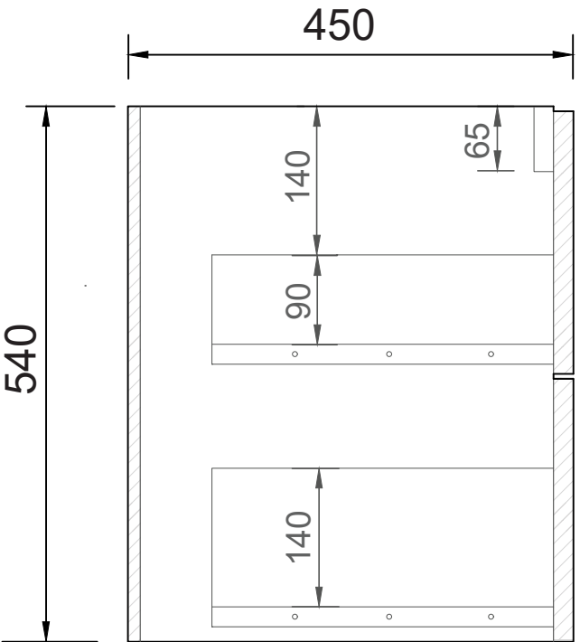
SIDE CROSS-SECTION
