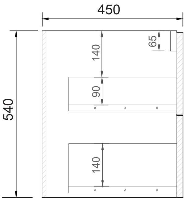
SIDE CROSS-SECTION
