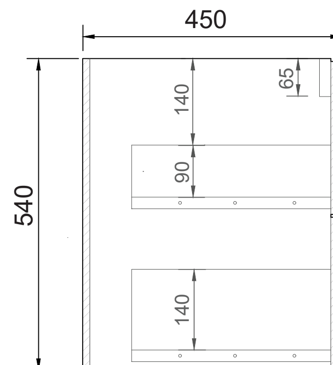
SIDE CROSS-SECTION
