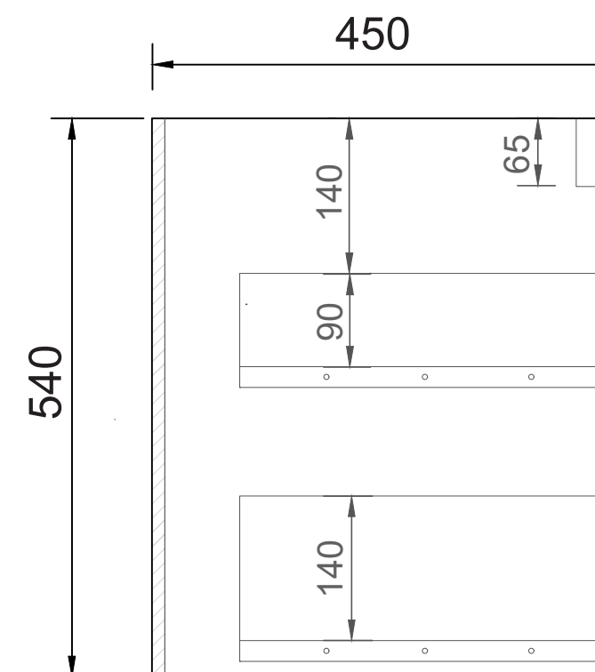
SIDE CROSS-SECTION
