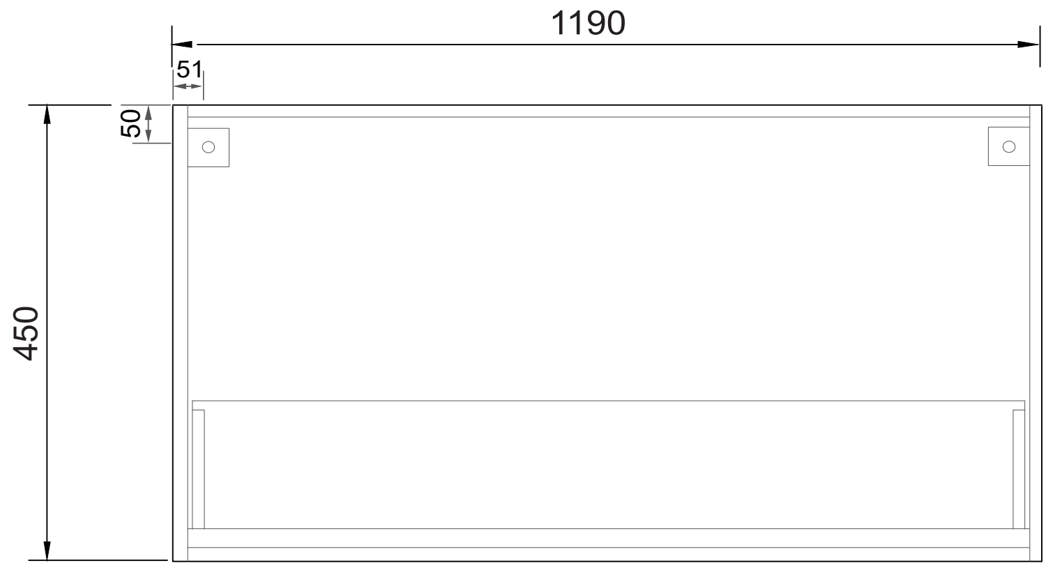
FRONT ELEVATION
