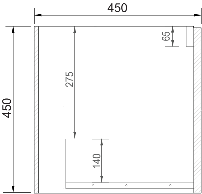
SIDE CROSS-SECTION
