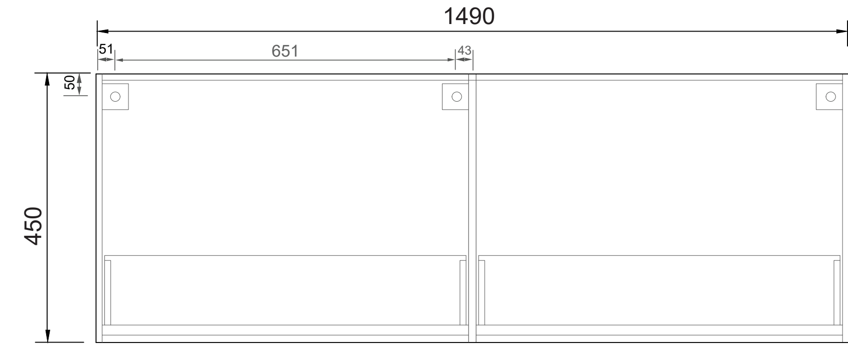
FRONT ELEVATION
