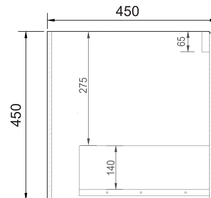
SIDE CROSS-SECTION
