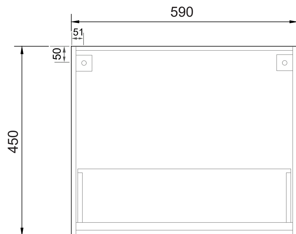
FRONT ELEVATION
