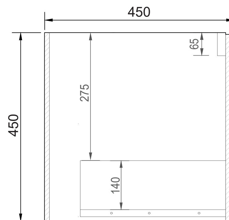
SIDE CROSS-SECTION
