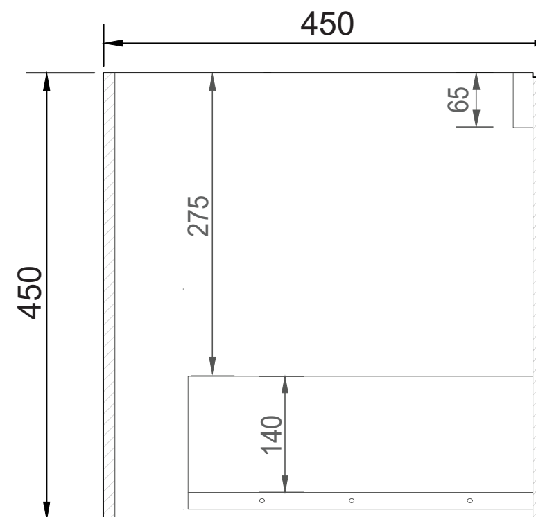
SIDE CROSS-SECTION
