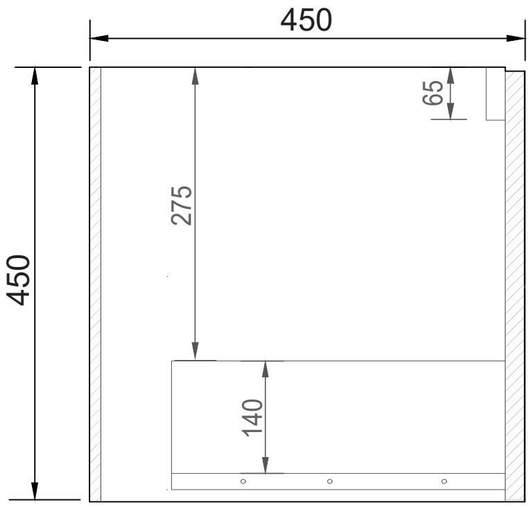
SIDE CROSS-SECTION
