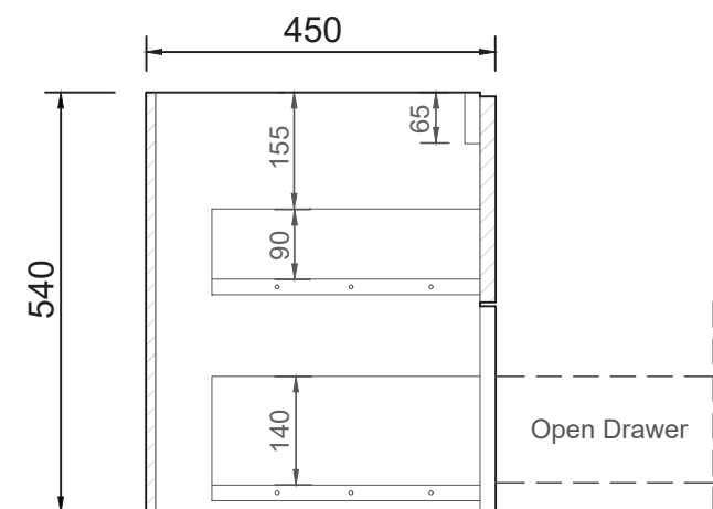
SIDE CROSS-SECTION
