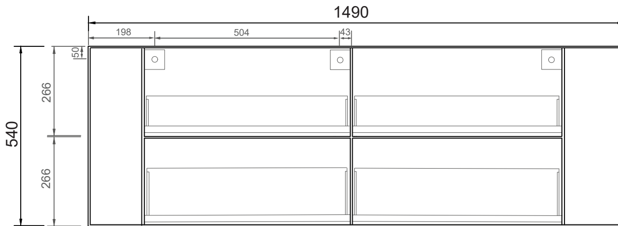
FRONT ELEVATION
