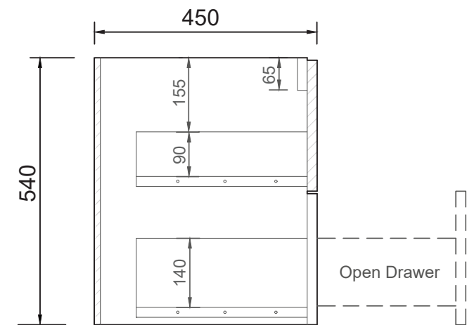
SIDE CROSS-SECTION
