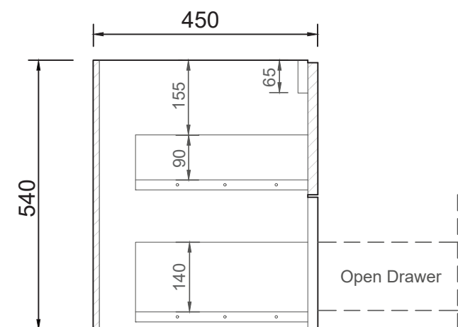
SIDE CROSS-SECTION
