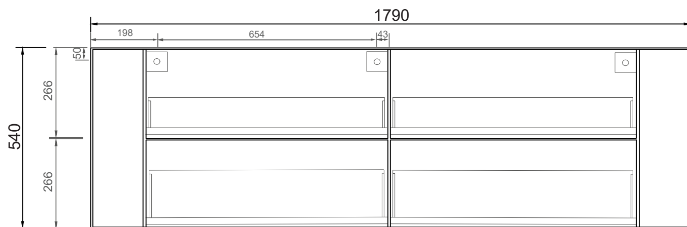
FRONT ELEVATION
