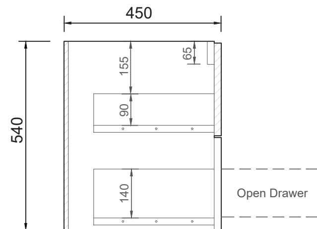
SIDE CROSS-SECTION
