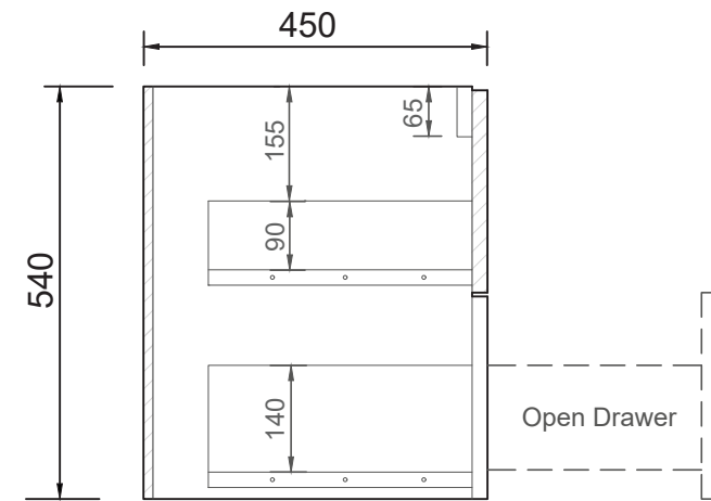
SIDE CROSS-SECTION
