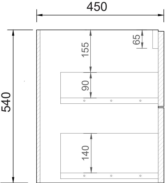
SIDE CROSS-SECTION
