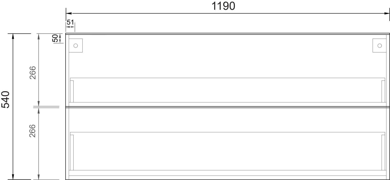
FRONT ELEVATION
