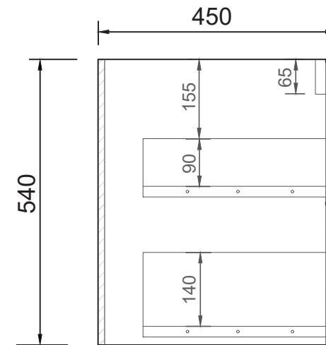
SIDE CROSS-SECTION
