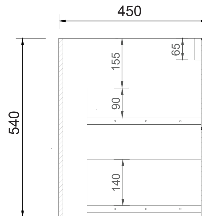
SIDE CROSS-SECTION
