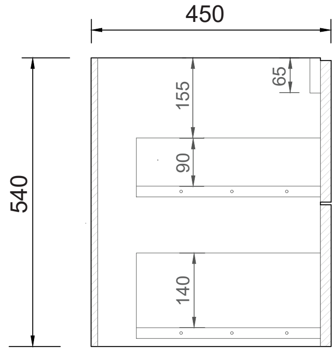
SIDE CROSS-SECTION
