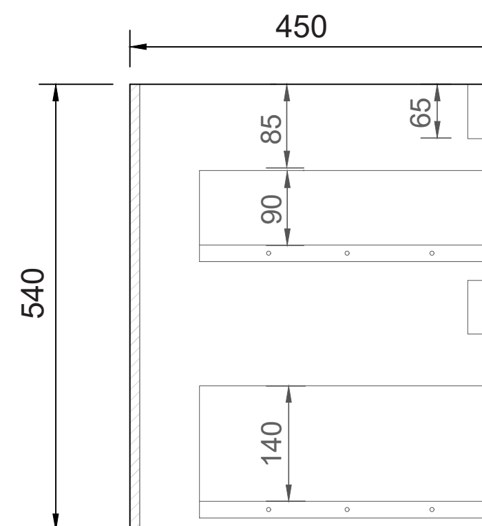
SIDE CROSS-SECTION
