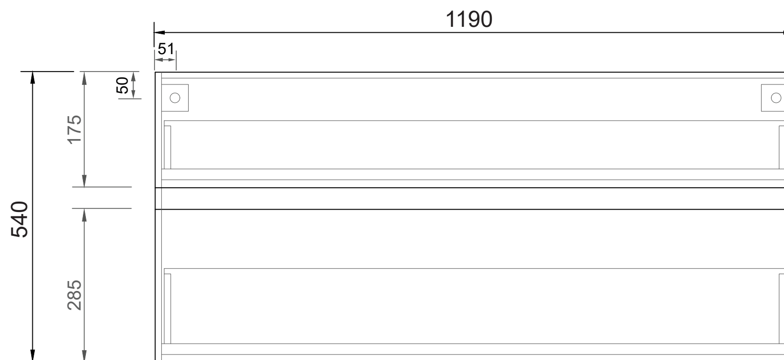
FRONT ELEVATION
