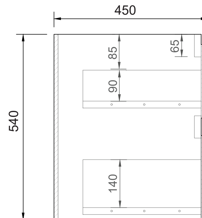
SIDE CROSS-SECTION
