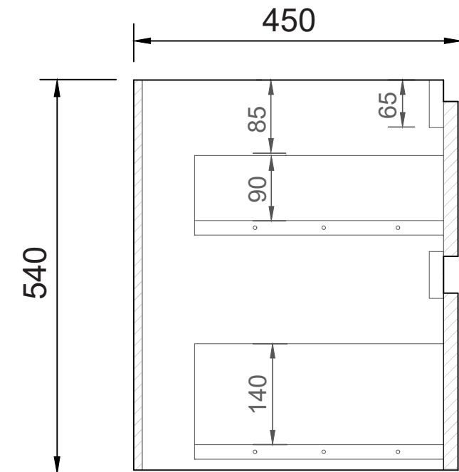
SIDE CROSS-SECTION
