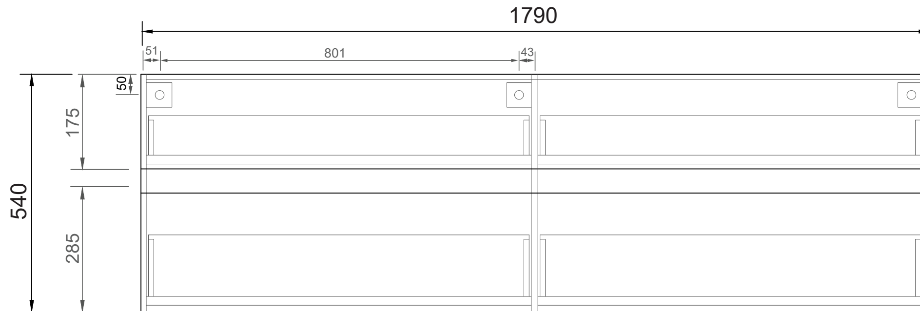
FRONT ELEVATION
