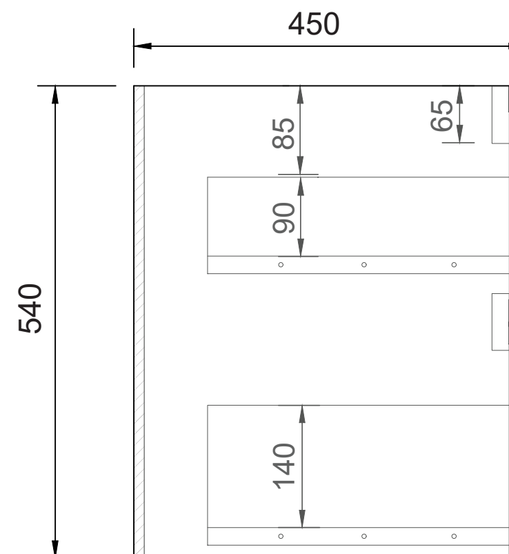
SIDE CROSS-SECTION
