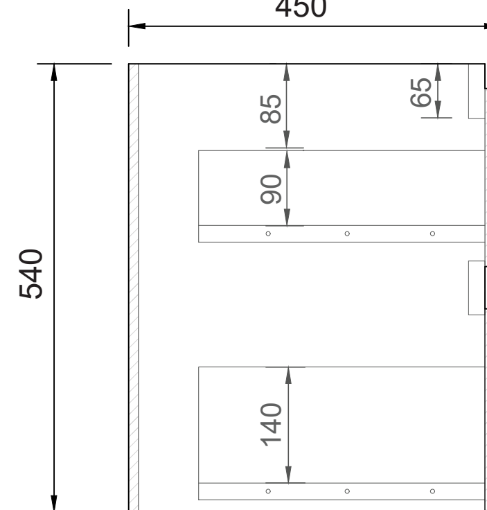
SIDE CROSS-SECTION
