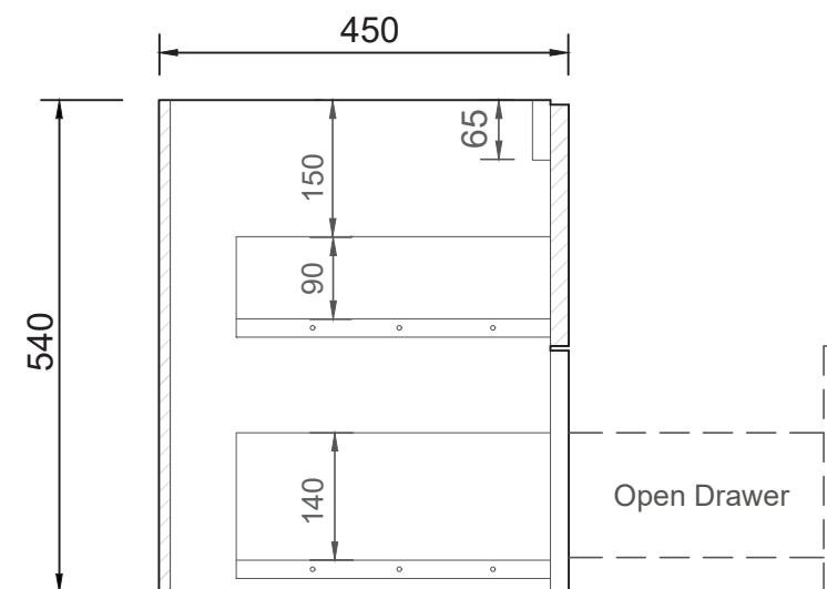
SIDE CROSS-SECTION
