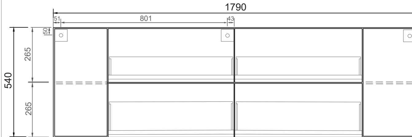
FRONT ELEVATION
