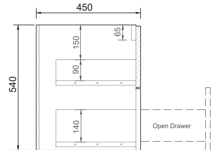
SIDE CROSS-SECTION
