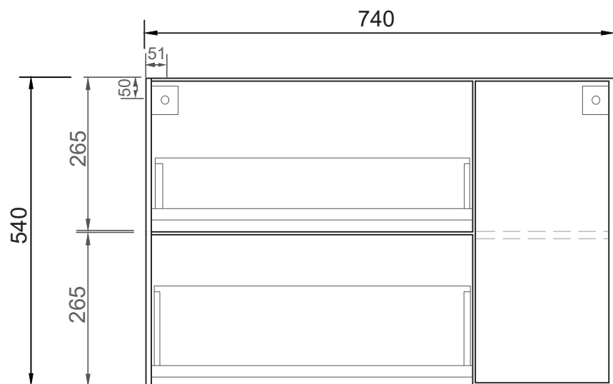
FRONT ELEVATION Right-hand side configuration.
