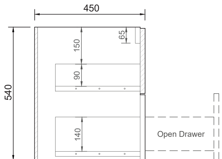
SIDE CROSS-SECTION
