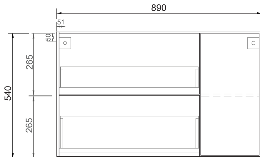
FRONT ELEVATION Right-hand side configuration.
