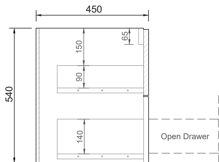
SIDE CROSS-SECTION Applies to both left-hand and right-hand configurations.
