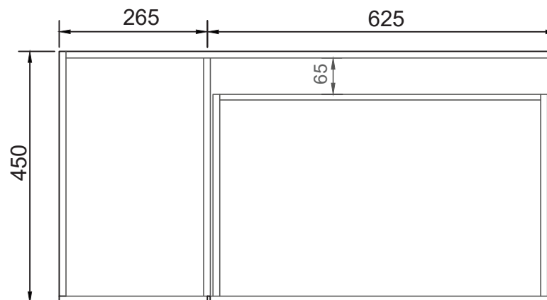
BIRD'S EYE VIEW Left-hand side configuration.
